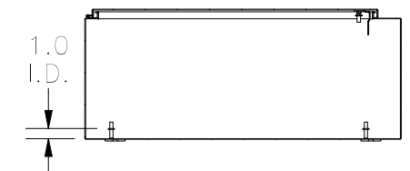
SECTION B-B (INSIDE TOP OF ENCLOSURE)
