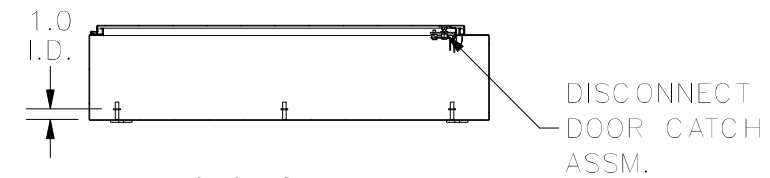
SECTION B-B (INSIDE TOP OF ENCLOSURE)
