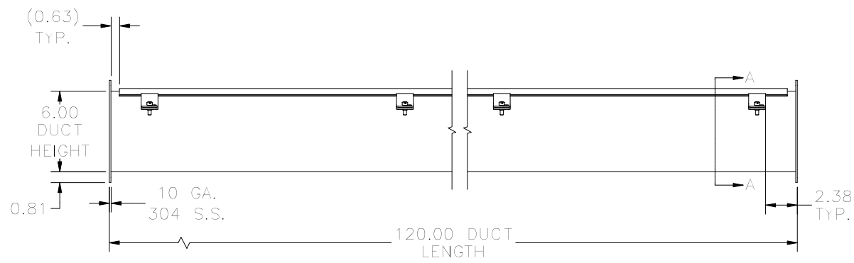
FRONT VIEW
