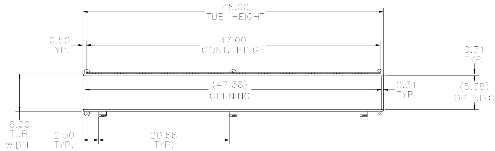
TOP VIEW (COVER REMOVED)
