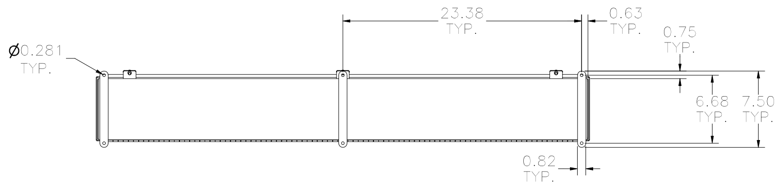
BOTTOM VIEW
