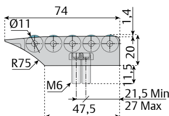
Version with 5 rollers
