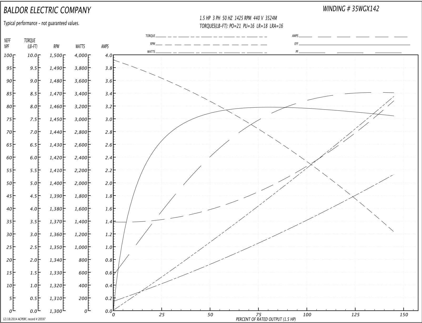
Performance Graph at 440V, 50Hz, 1.5HP Typical performance - Not guaranteed values
