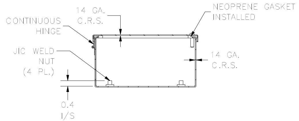
SECTION B-B VIEW (INSIDE TOP OF ENCL.)
