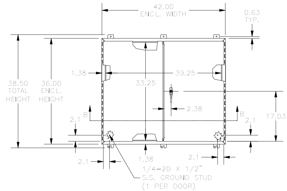
FRONT VIEW
