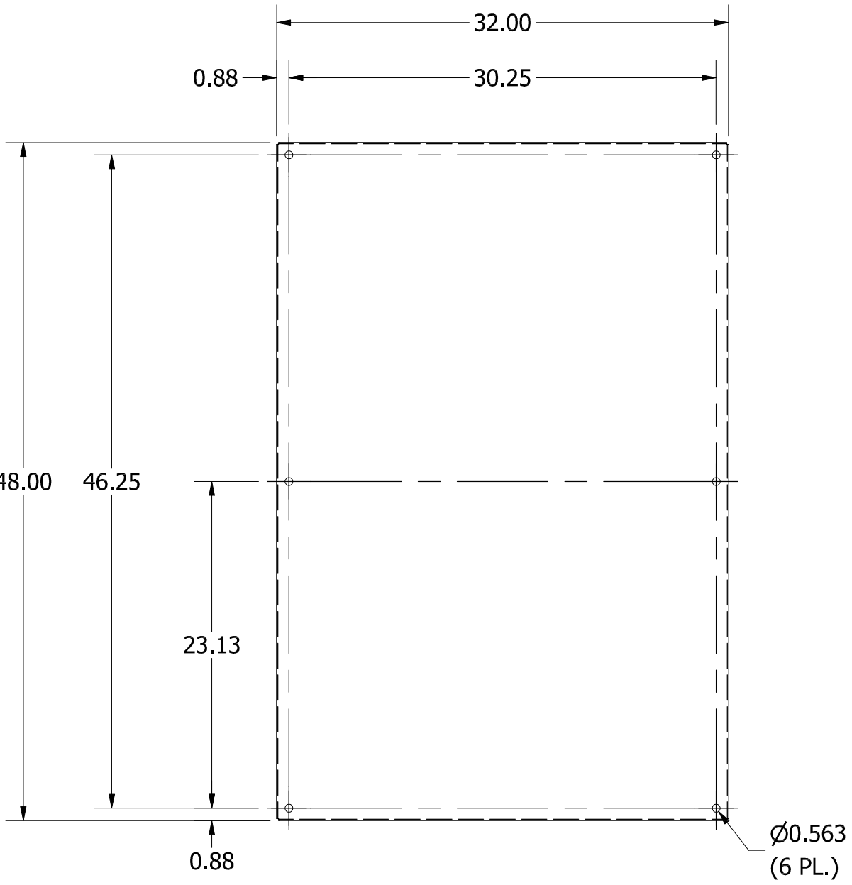
FRONT VIEW
