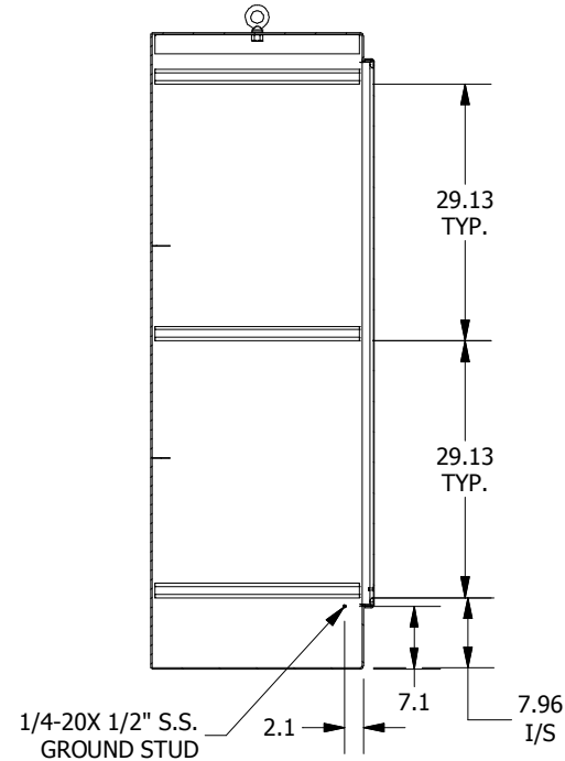
SECTION B-B (INSIDE RIGHT OF ENCL.)
