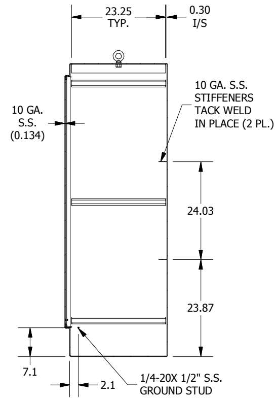
SECTION A-A (INSIDE LEFT OF ENCL.)
