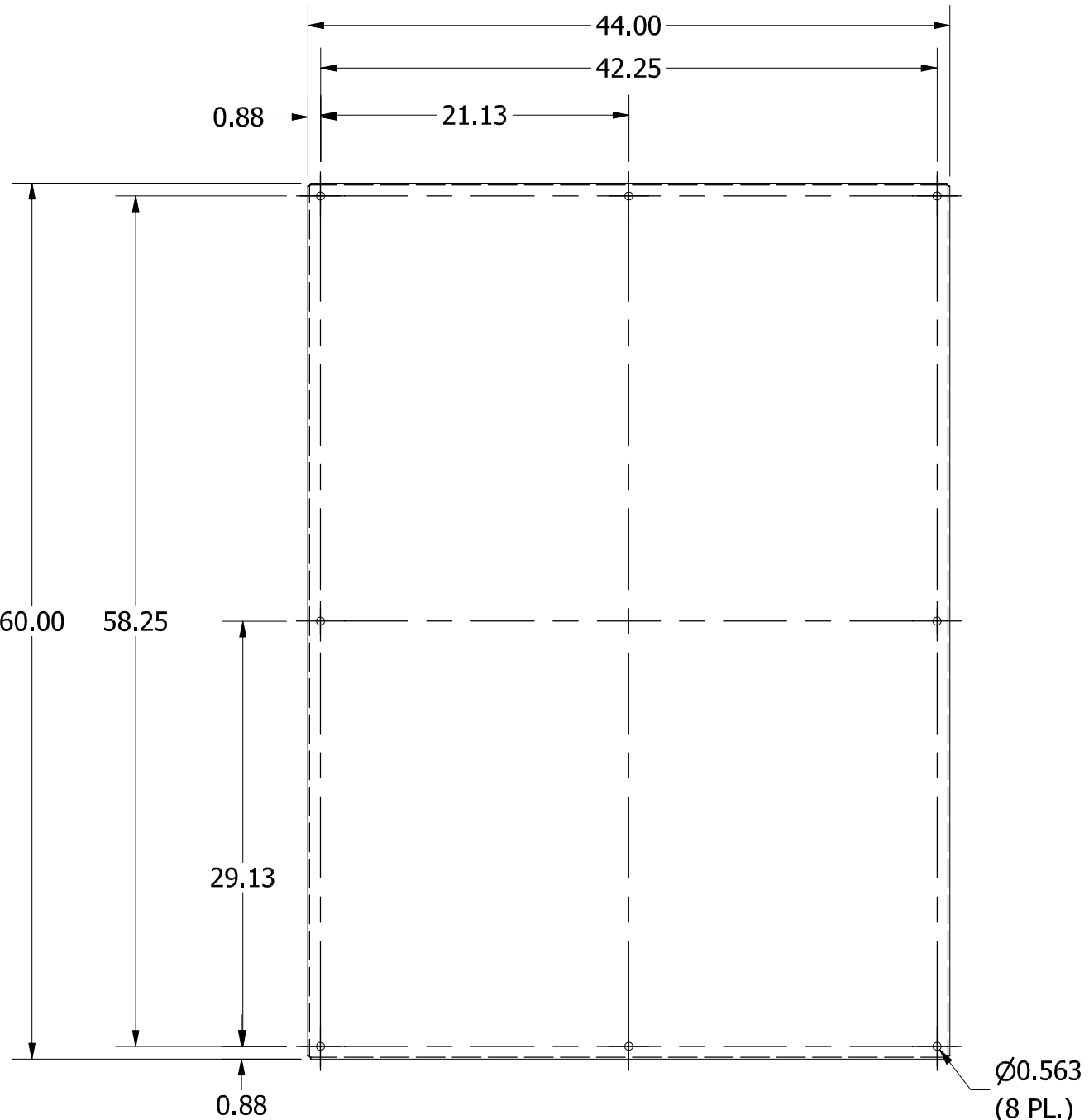
FRONT VIEW
