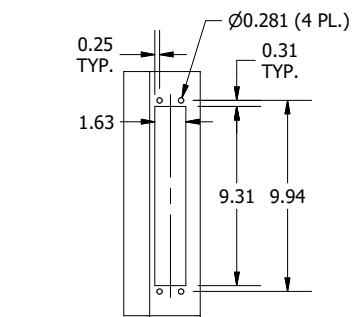
DETAIL L (DISCONNECT CUTOUT DETAIL)
