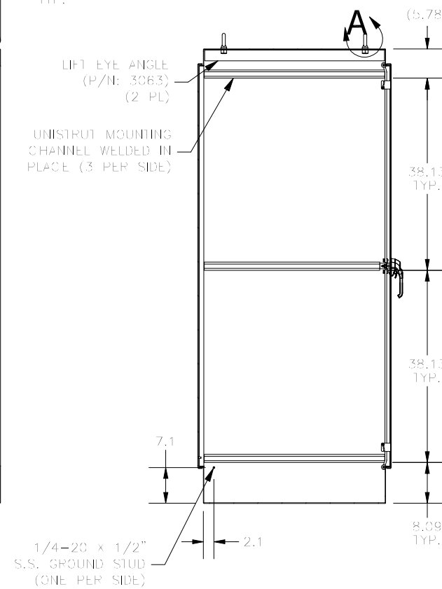
SECTION A-A (INSIDE SIDE OF ENCL.) (TYP.)
