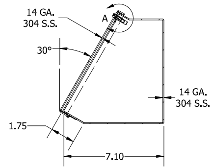
SECTION A-A VIEW (INSIDE LEFT OF ENCL.)
