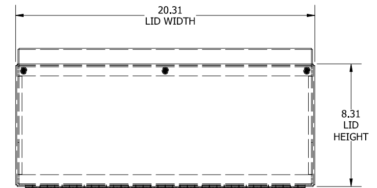
SECTION B-B (STRAIGHT AHEAD VIEW OF LID)
