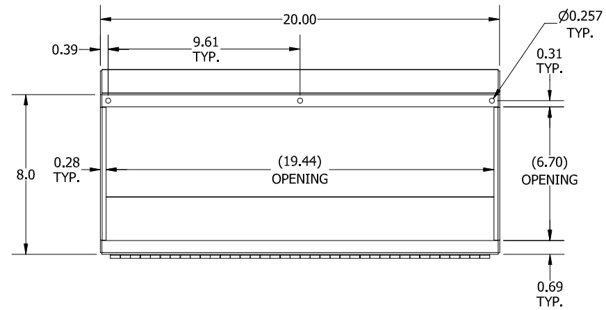
VIEW B-B (LID ASSM. REMOVED)
