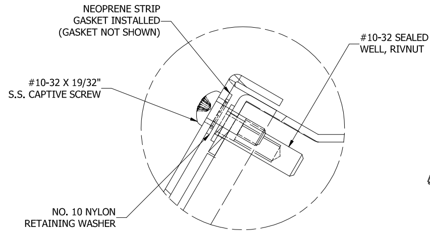
DETAIL A (3 PL.) (LID ATTACHMENT DETAIL)
