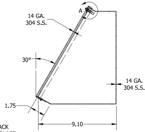
SECTION A-A VIEW (INSIDE LEFT OF ENCL.)
