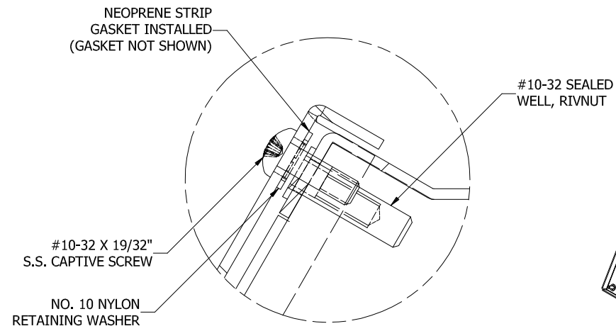
DETAIL A (3 PL.) (LID ATTACHMENT DEATIL)
