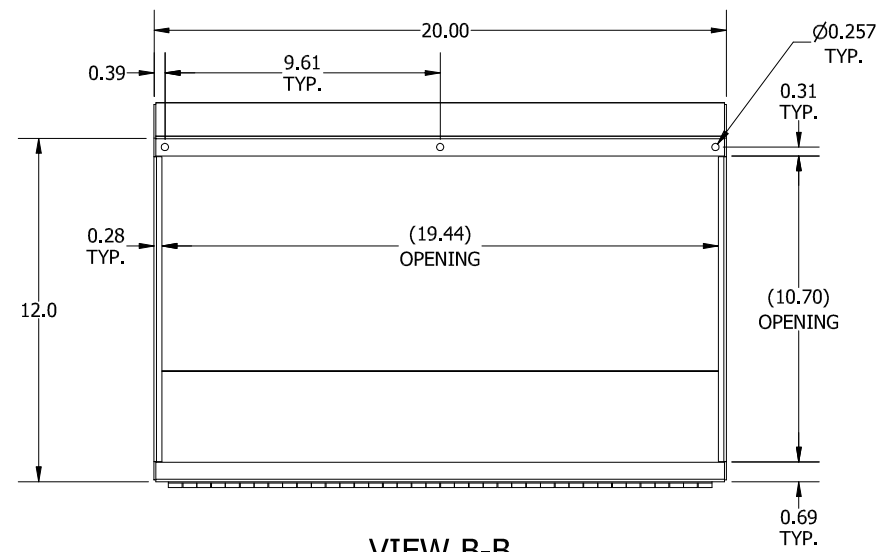
VIEW B-B (LID ASSM. REMOVED)
