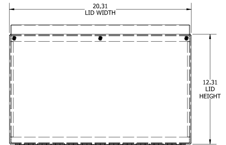
SECTION B-B (STRAIGHT AHEAD VIEW OF LID)
